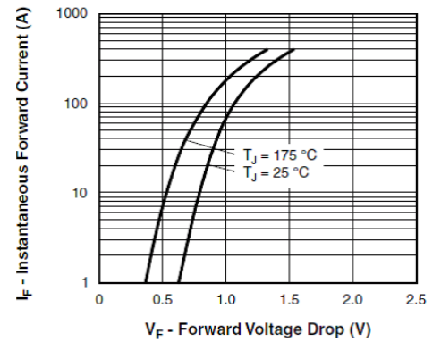
UFB280FA40 typical forward voltage drop characteristics
