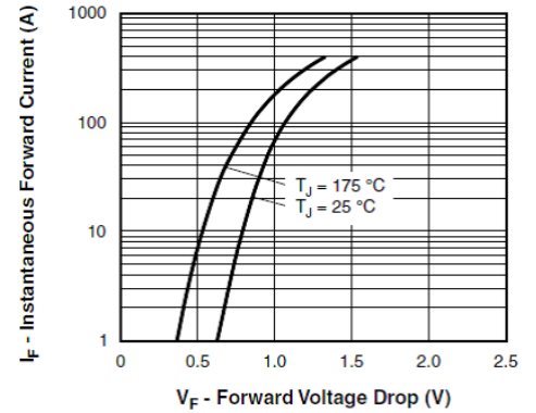
UFB280FA40 typical forward voltage drop characteristics
